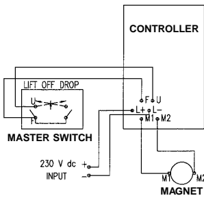
SYSTEMS DIAGRAM
