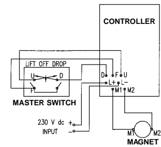
SYSTEMS DIAGRAM
