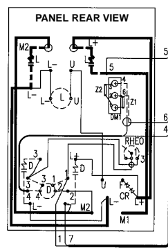
WIRING DIAGRAM
