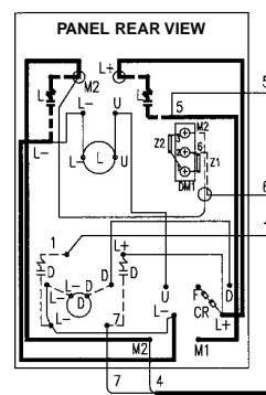
WIRING DIAGRAM
