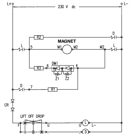
SCHEMATIC DIAGRAM
